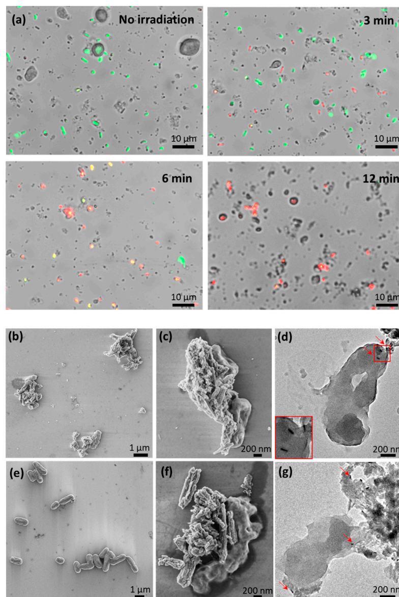
Figure 5. Light and electron microscopy imaging of the antibacterial photothermal effect exerted by AuNR-Ab-HNTs hybrids—mixtures containing AuNR-Ab-HNTs hybrids and E. coli irradiated using a 808 nm laser ( 4 \text{ W cm}^{-2} ) and imaged using (a) overlay of bright-field and fluorescence microscopy after irradiation time of 0, 3, 6, and 12 min (upper panel left to right and bottom panel left to right, respectively). Bacteria were labeled with Live/Dead staining: Green—Syto9, Red—propidium iodide; (b,c,f) SEM for 12 min irradiation; and (d,g) TEM for 12 min irradiation. (High contrast gold nanorods are indicated by red arrows. The red frame inset depicts higher magnification of the region of interest marked with a red rectangle.) (e) SEM micrograph of untreated E. coli cells.
