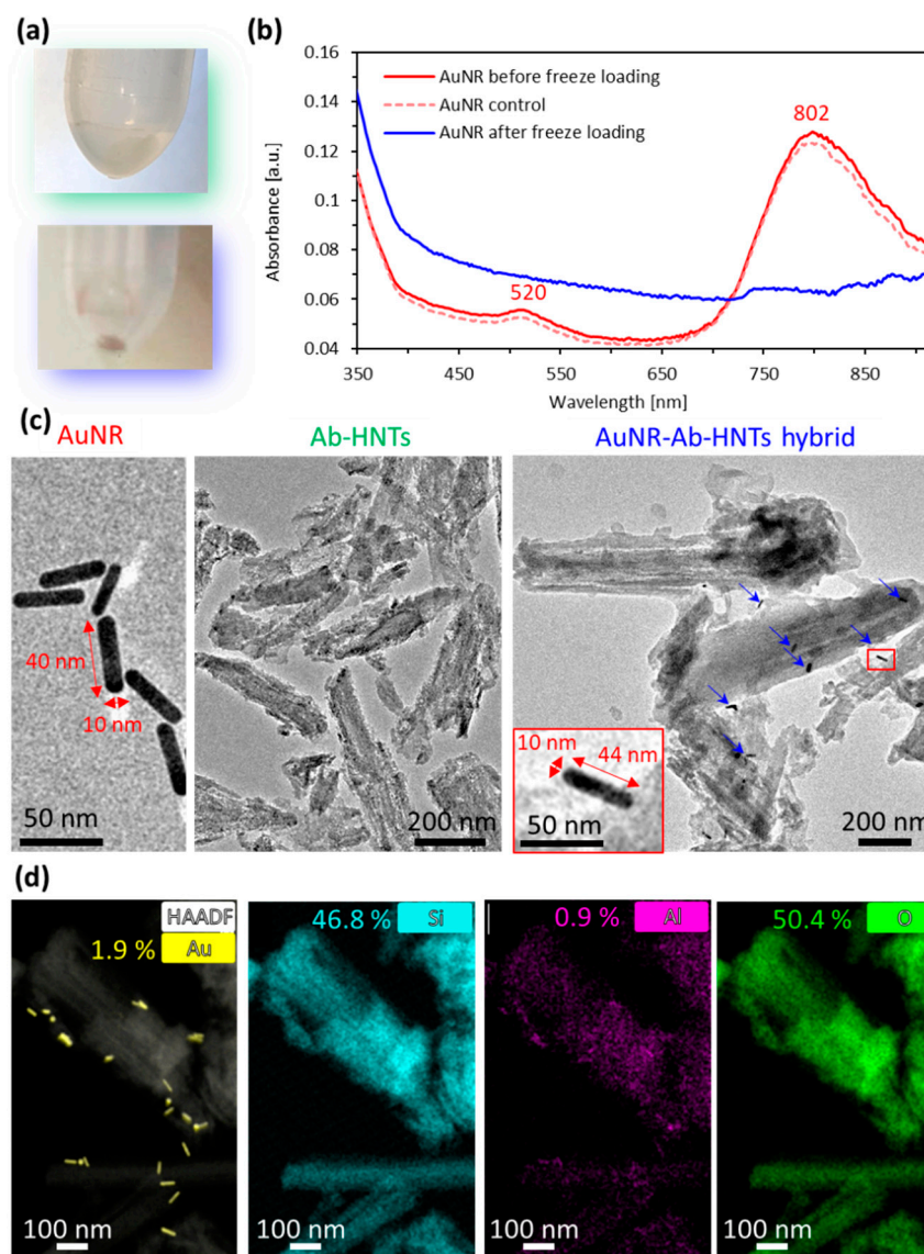
Figure 2. Incorporation of AuNRs onto Ab-HNTs. (a) Photographs of the Ab-functionalized HNTs (top panel) and AuNR-Ab-HNTs hybrids (bottom panel); (b) UV-Vis spectra at 350–920 nm of AuNR suspension before and after freezing-induced loading (red and blue traces, respectively), and a control of an AuNR suspension with no HNTs similarly processed (light red dashed trace). (c) TEM micrographs of: Left panel—free AuNR, red arrows indicate the measured dimensions of a gold nanorod with values detailed next to each corresponding arrow; Middle panel—Ab-HNTs without AuNRs; Right panel—AuNR-Ab-HNTs hybrids, blue arrows mark loaded AuNR, and red-frame inset depicts high magnification of the region of interest marked with a red rectangle. (d) STEM-EDX micrographs of AuNR-Ab-HNTs hybrid from left to right: an overlay of high-angle annular dark-field (HAADF) detector and Au elemental mapping; separate elemental mapping for Si, Al, and O. The measured wt.% of each element is indicated next to the element symbol.
