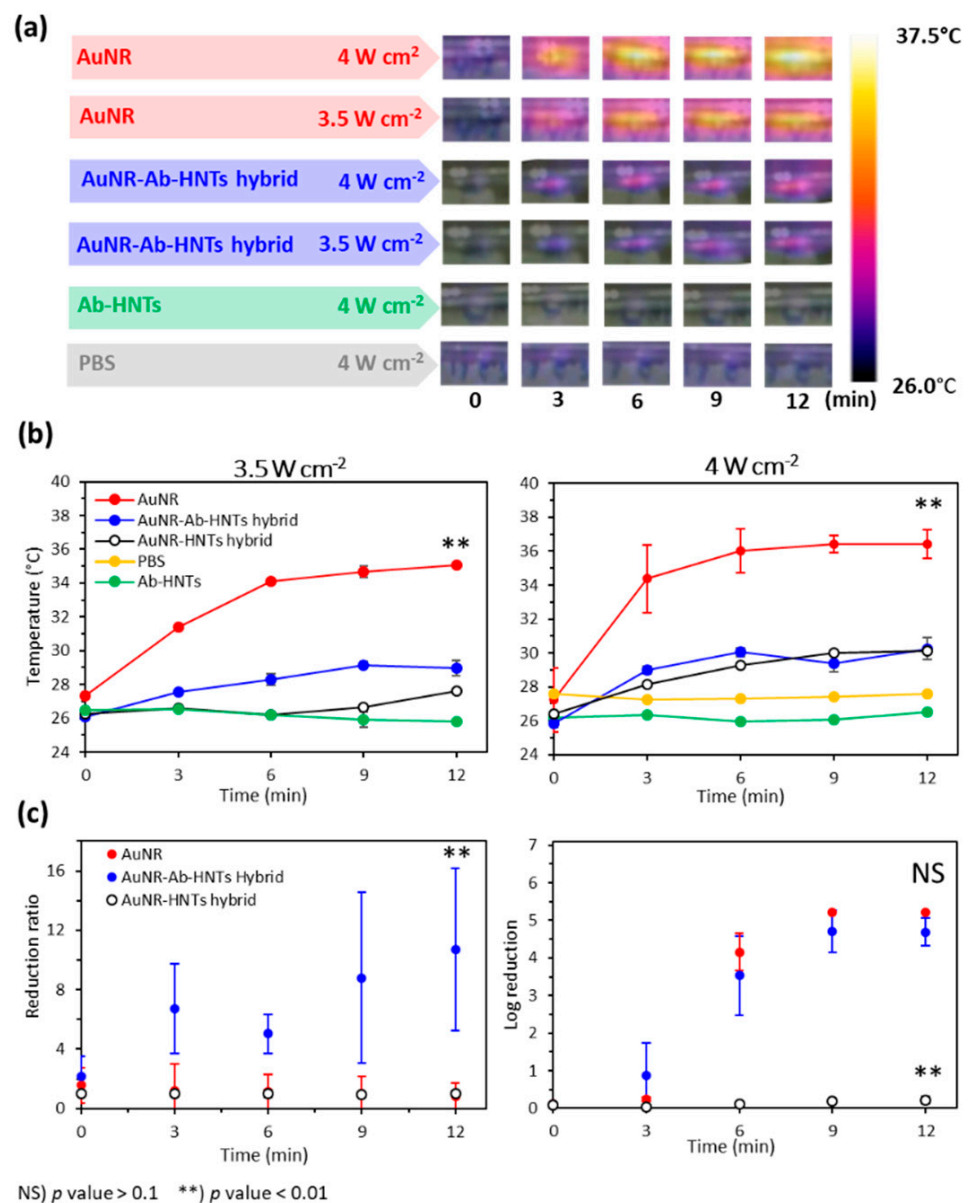
Figure 4. Antibacterial photothermal treatment (APTT) of AuNR-Ab-HNTs hybrids compared with free AuNRs. (a) Examples of thermal camera images. (b) Temperature measurements using the thermal camera, as a function of irradiation (808 nm) time at a power density of 3.5 and 4 W cm -2 (left and right panel, respectively) for AuNR-Ab-HNTs hybrids (blue), free AuNRs (red), Ab-HNTs without AuNRs (green), AuNR-HNTs hybrid without antibody (black with hollow marker), and PBS control (yellow). (c) Antibacterial effect measured by plate count as a function of irradiation (808 nm) and time, at a power density of 3.5 and 4 W cm -2 for left and right panels, respectively (color scheme similar to all other results in this figure). Error bars represent SD ( n = 3 ). NS: p -value > 0.1; **: p -value < 0.01 according to a two-tailed t -test.
